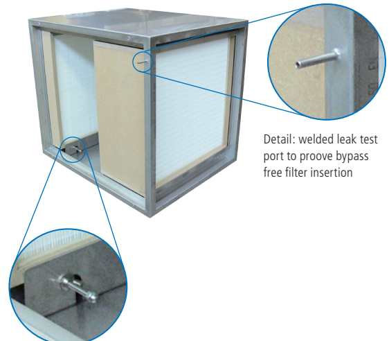
Detail: Filter Mounting with rapid clamping
